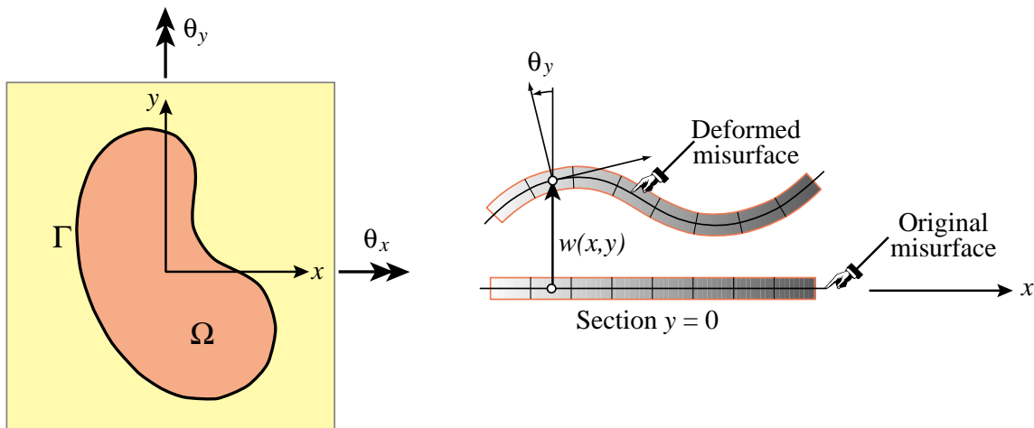
Figure 24.3. Kinematics of a Kirchhoff plate. Lateral deflection w greatly exaggerated for visibility. In practice w \ll h for the Kirchhoff model to be valid.
