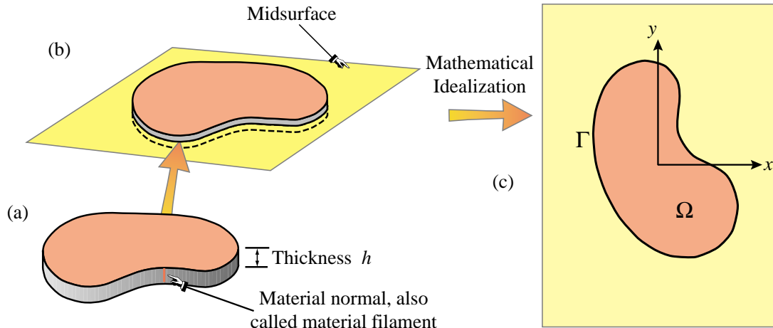
Figure 24.2. Idealization of plate as two-dimensional problem.
