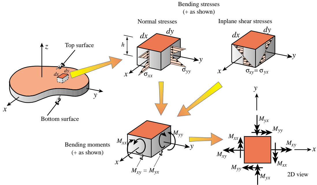
Figure 24.4. Bending stresses and moments in a Kirchhoff plate.
