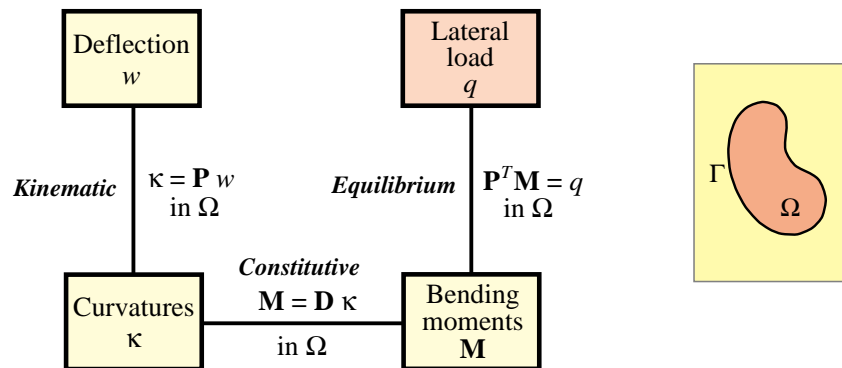
Figure 24.8. Strong Form diagram of the field equations of the Kirchhoff plate. Boundary condition links omitted.
