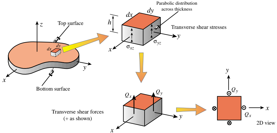
Figure 24.5. Transverse shear forces and stresses in a Kirchhoff plate.
