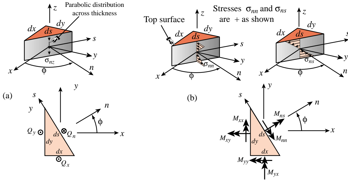
Figure 24.7. Skew plane sections in Kirchhoff plate.
